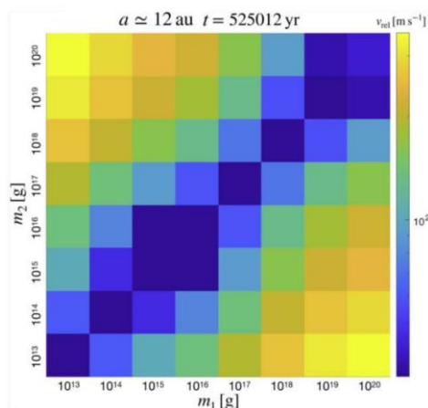
Fig.1: Relative velocity between particles of m_1 and m_2 near 12 au at t=525012 yr.
