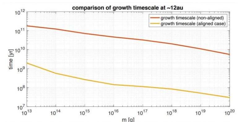
Fig.2: Growth timescales with orbital alignment (yellow) and without orbital alignment (red) near 12 au.
